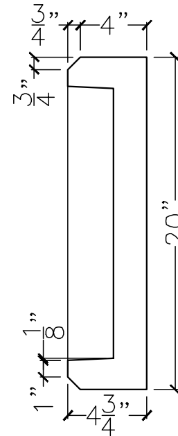
SECTION VIEW
