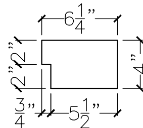
SECTION VIEW
