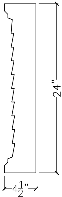
SECTION VIEW
