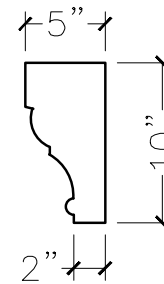
SECTION VIEW
