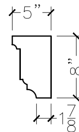
SECTION VIEW
