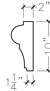
SECTION VIEW
