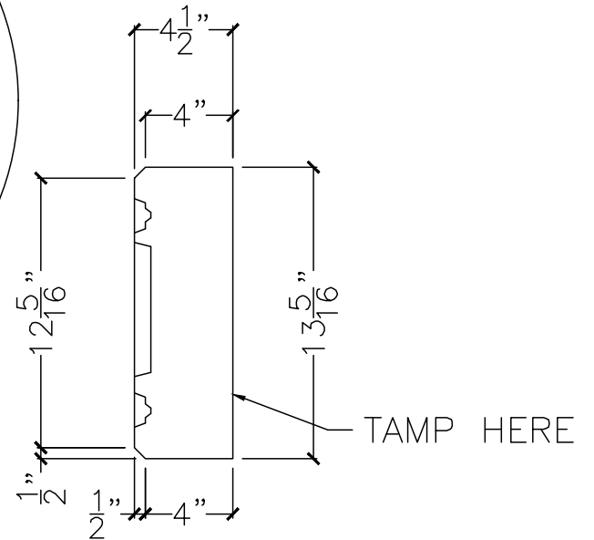
SECTION VIEW
