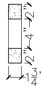
SECTION VIEW
