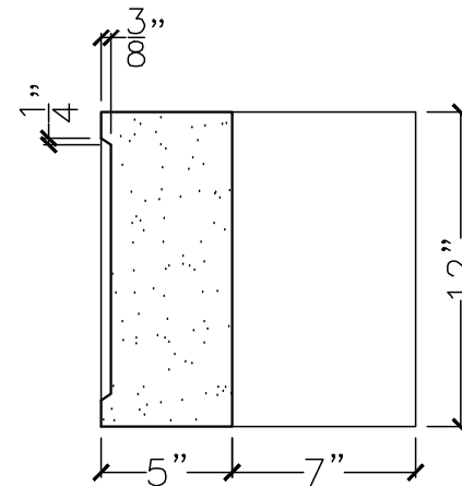
SECTION VIEW
