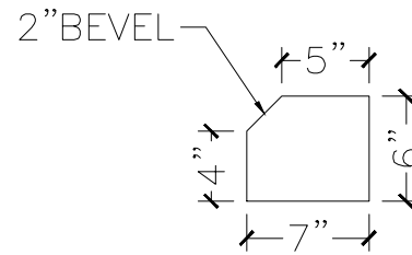
SECTION VIEW
