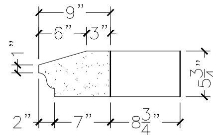
SECTION VIEW
