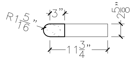
SECTION VIEW
