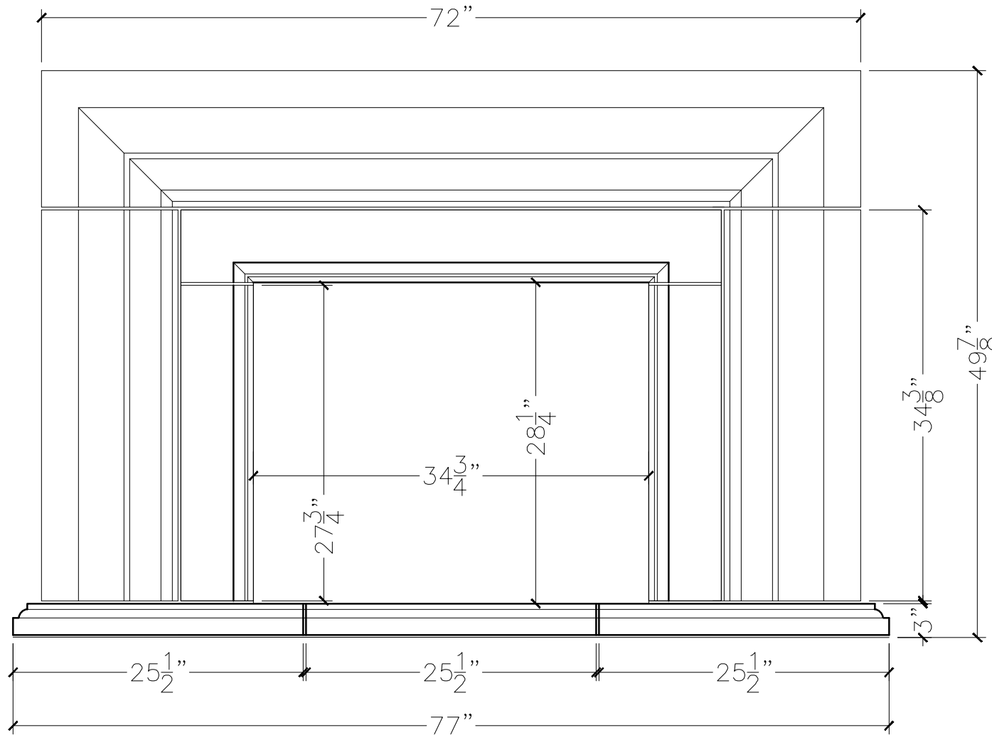
FRONT VIEW
