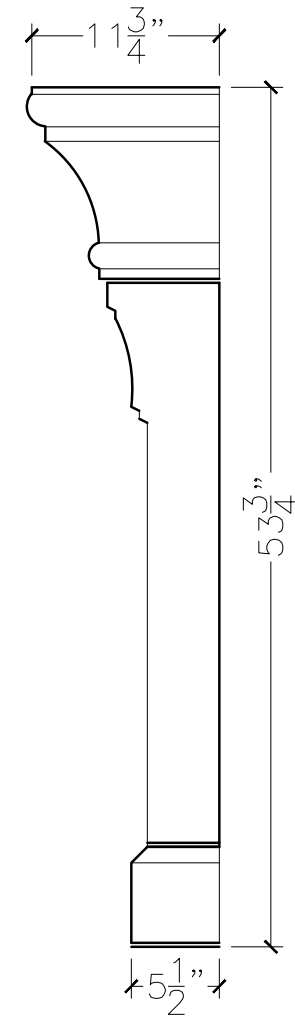
SECTION
