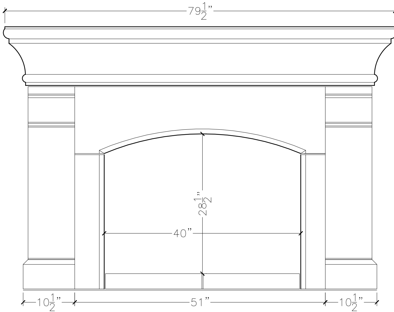
FRONT VIEW
