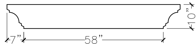
SECTION VIEW
