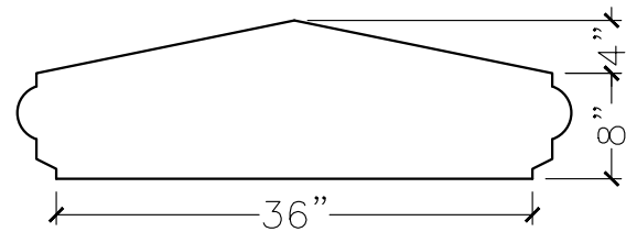
SECTION VIEW
