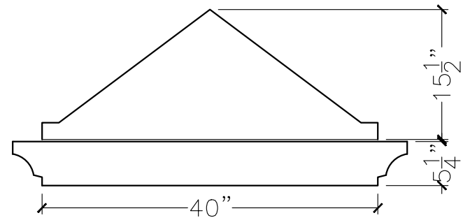
SECTION VIEW
