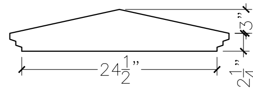
SECTION VIEW
