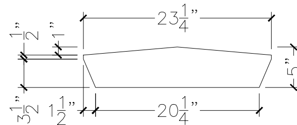
SECTION VIEW
