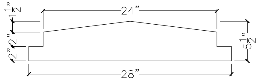
SECTION VIEW
