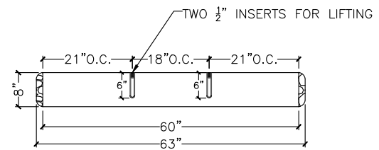
SECTION VIEW
