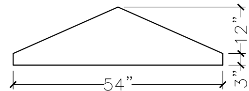
SECTION VIEW
