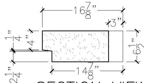
SECTION VIEW
