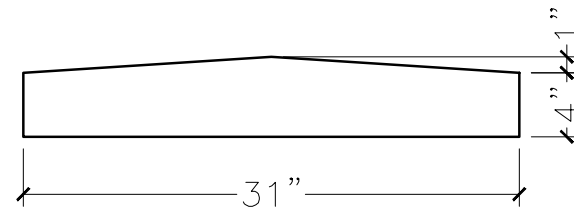
SECTION VIEW
