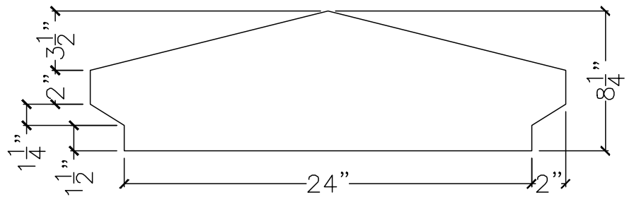
SECTION VIEW
