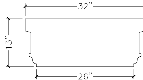
SECTION VIEW
