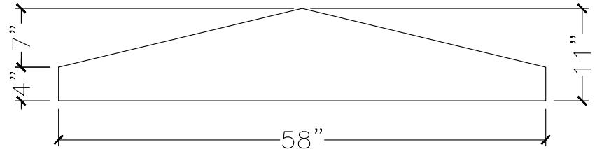
SECTION VIEW
