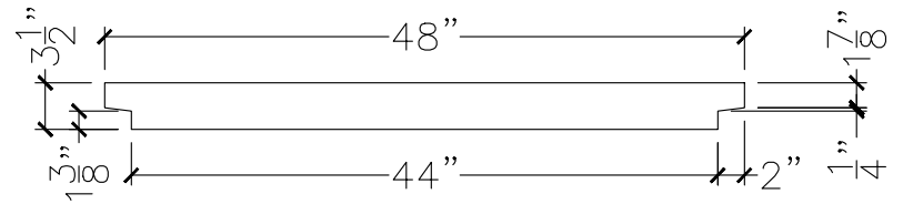
SECTION VIEW
