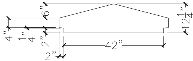
SECTION VIEW
