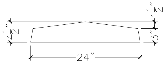
SECTION VIEW
