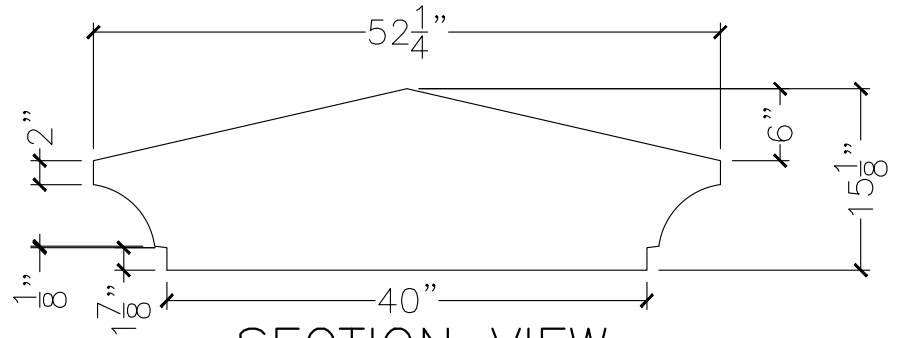
SECTION VIEW
