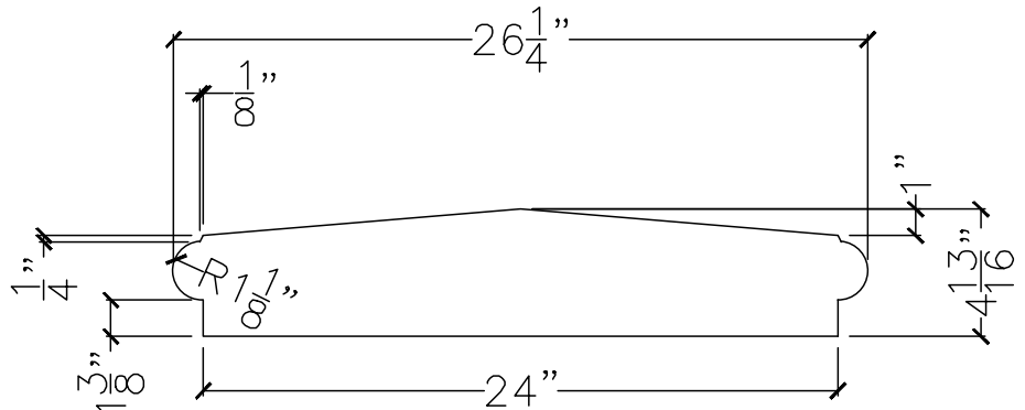
SECTION VIEW
