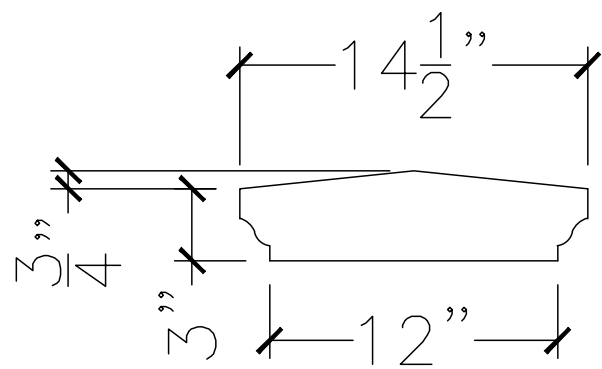
SECTION VIEW
