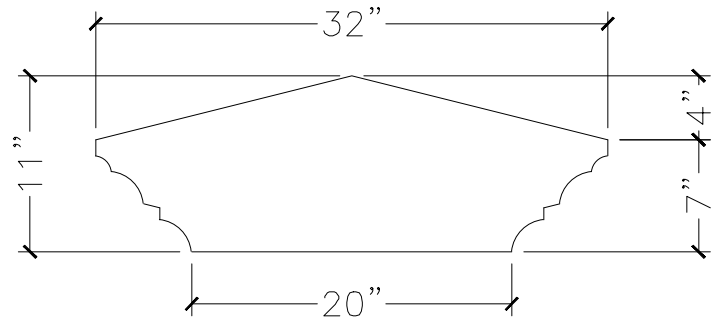
SECTION VIEW
