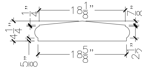
SECTION VIEW
