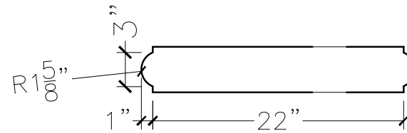
SECTION VIEW
