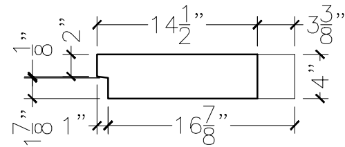
SECTION VIEW
