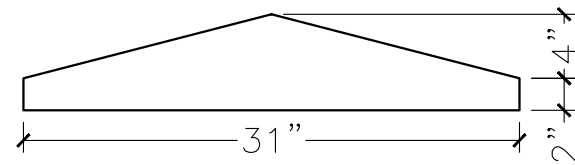
SECTION VIEW
