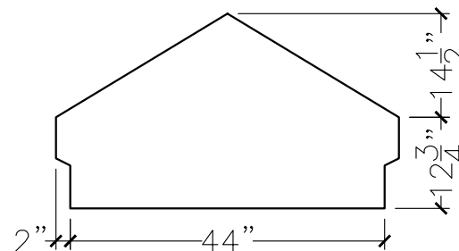
SECTION VIEW
