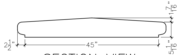
SECTION VIEW
