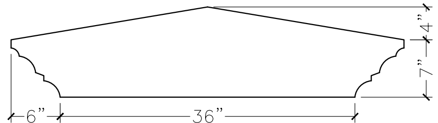
SECTION VIEW
