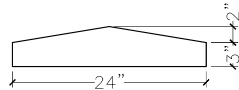
SECTION VIEW
