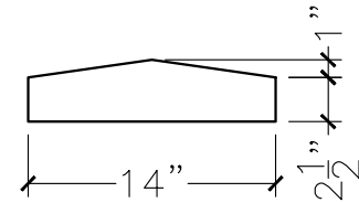
SECTION VIEW
