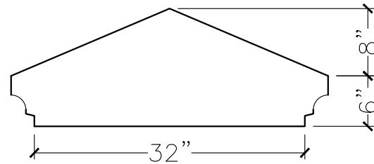
SECTION VIEW
