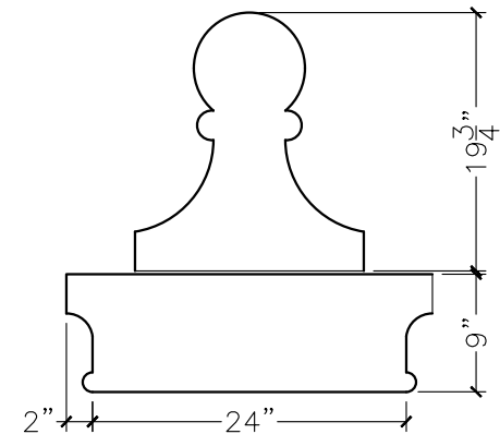
SECTION VIEW
