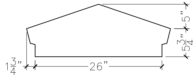
SECTION VIEW
