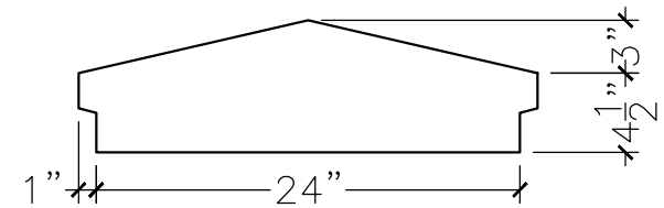
SECTION VIEW
