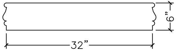
SECTION VIEW
