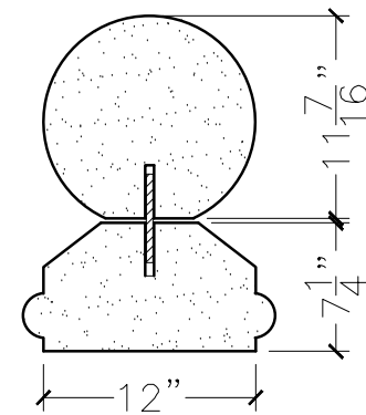
SECTION VIEW
