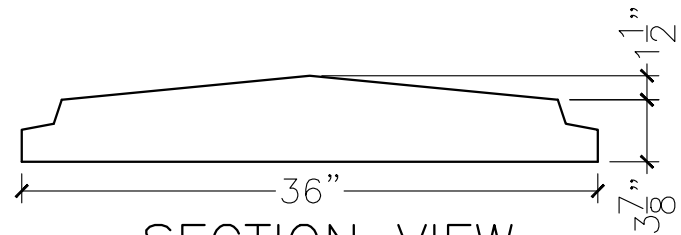
SECTION VIEW
